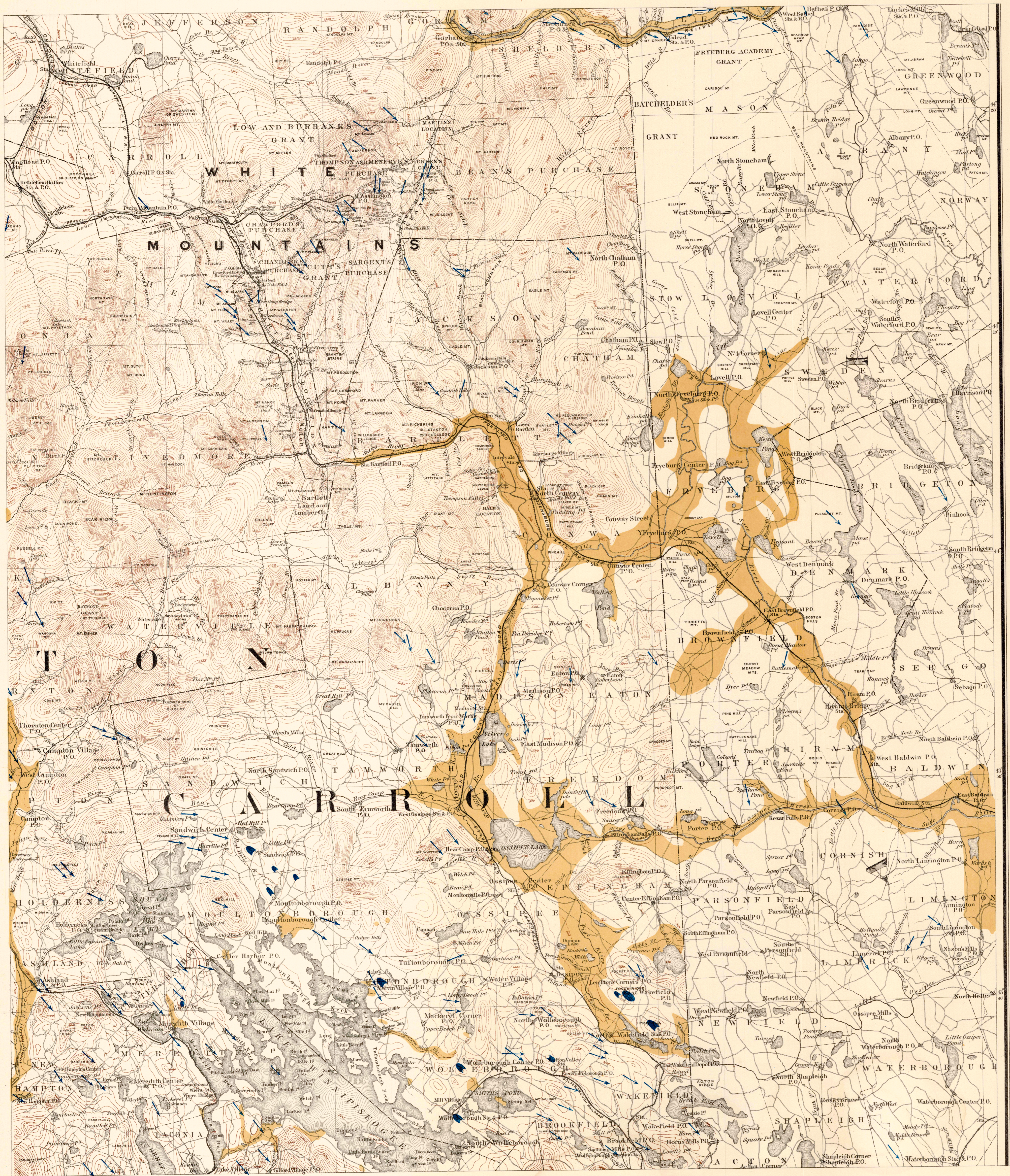
→ Glacial Striae ● Lenticular Hills and Slopes of Till Modified Drift
