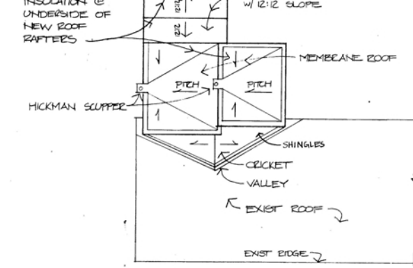
① UPPER ROOF PLAN
